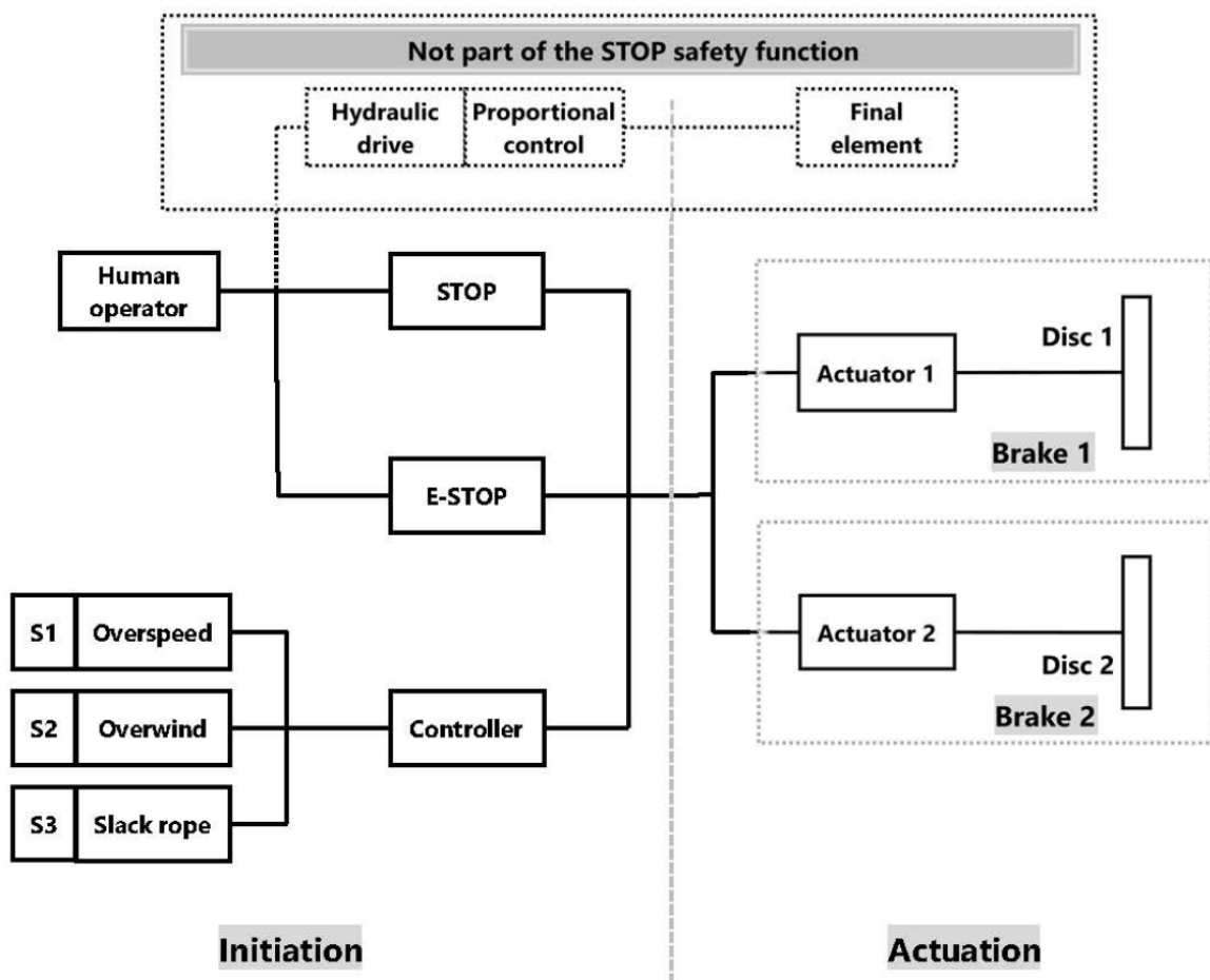
Figure 6. Depicts a hypothetical shaft sinking winder system as a block diagram.
