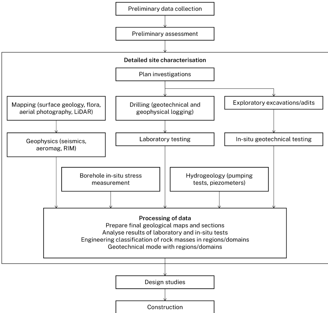
Figure 1. Flowchart example of an initial site characterisation exercise
