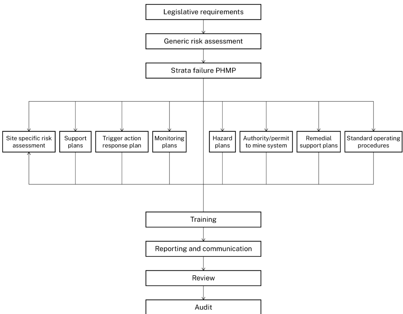
Figure 3. Typical strata failure hazard management plan framework
